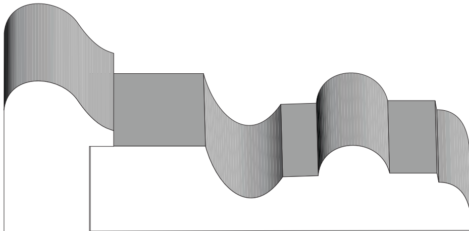
BA 1563 1-1/8" x 1-9/16"
