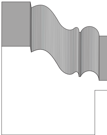
BA 2003 1-1/2" x 1-13/16"
