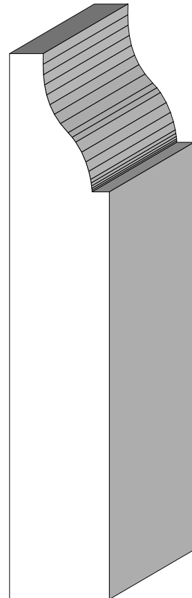
BA 506 3/4" x 4"
