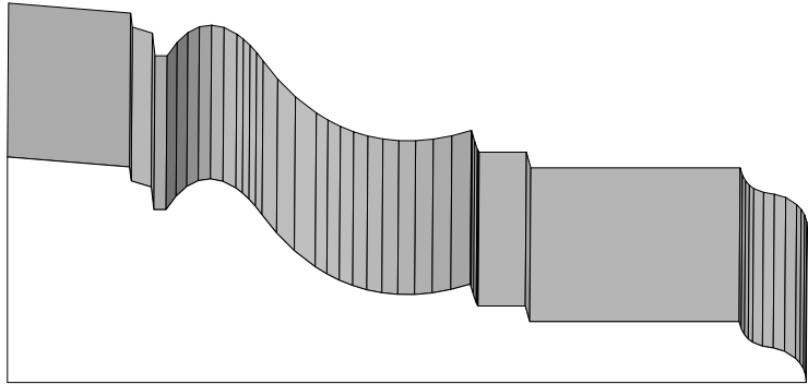
BA 675 (Similar to BA 1220 & 1221) 1-1/8" x 3-13/16"
