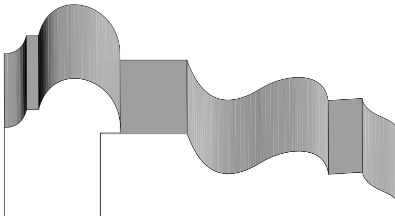
BA 1500 1-3/16" x 1-3/8"
